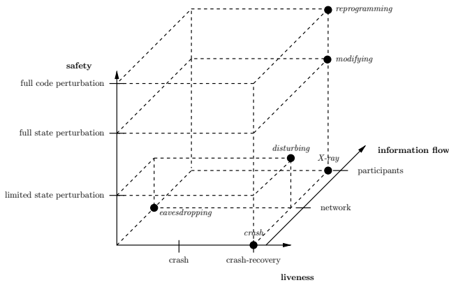
Figure 2: Embedding intervention levels in a general attacker model.
