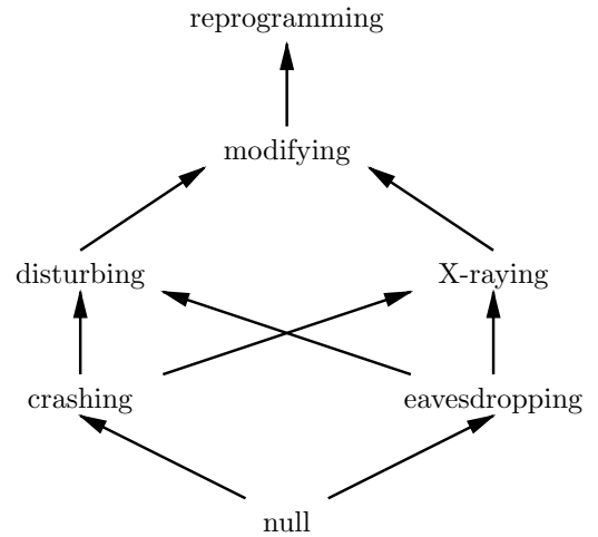
Figure 1: Lattice of intervention levels, where X \rightarrow Y means Y includes all attacker behavior of X .
